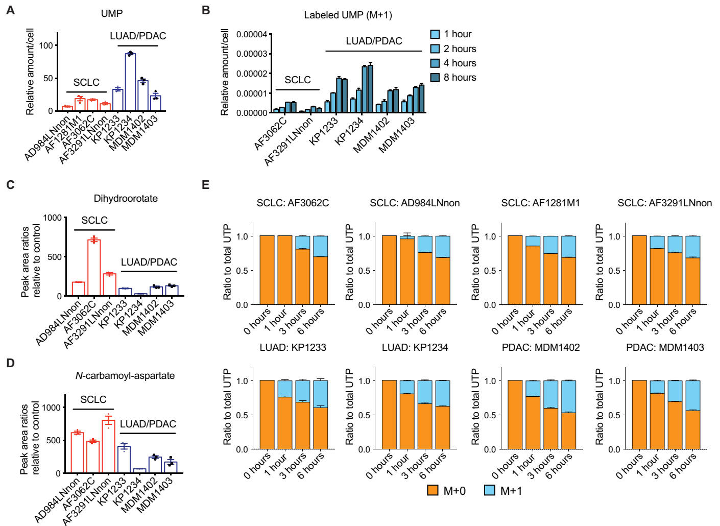
Fig. 2. SCLC cells exhibit lower flux through the de novo pyrimidine synthesis pathway compared with LUAD/PDAC cells. (A) Baseline uridine monophosphate (UMP) concentrations in untreated SCLC, LUAD, and PDAC cell lines, as measured by liquid chromatography–mass spectrometry. Data are shown as relative amounts normalized to cell number, after absolute quantification using external UMP standards ( n = 3 technical replicates per cell line). (B) Concentrations of newly synthesized UMP (M+1) in untreated SCLC, LUAD, and PDAC cell lines at the indicated time points after the start of ^{15}\text{N} -glutamine labeling. Data are shown as relative amounts normalized to pool size per cell ( n = 3 technical replicates per condition). (C and D) Dihydroorotate (C) and N -carbamoyl-aspartate (D) concentrations in SCLC, LUAD, and PDAC cell lines 6 hours after treatment with 1\ \mu\text{M} brequinar. Data are normalized to untreated controls and adjusted for cell number ( n = 3 technical replicates per cell line). (E) Fractions of newly synthesized (M+1) and preexisting (M+0) uridine triphosphate (UTP) in SCLC, LUAD, and PDAC cell lines treated with 1\ \mu\text{M} brequinar at the indicated time points after the start of ^{15}\text{N} -glutamine labeling. Data are normalized to total UTP concentrations in each cell line ( n = 3 technical replicates per condition). All data are presented as means \pm SEM.
