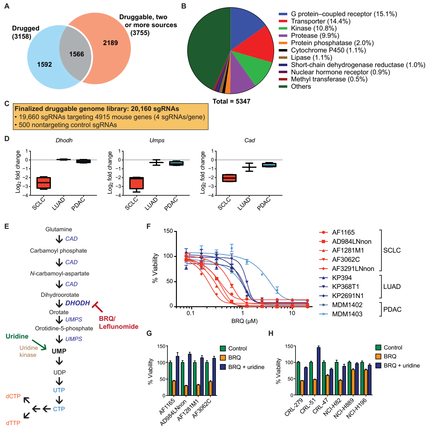
Fig. 1. SCLC cells are sensitive to disruption of the de novo pyrimidine synthesis pathway. (A) Number of genes in each category in the druggable genome library. (B) Composition of genes in the druggable genome library by gene category. (C) Breakdown of the total number of sgRNAs in the druggable genome library. (D) Gene scores (log 2 fold change) for the indicated genes for SCLC ( n = 4 biological replicates), LUAD ( n = 2 biological replicates), and PDAC ( n = 4 biological replicates). Data are presented as median gene scores, with boxes denoting the interquartile range and bars denoting the range. (E) Pyrimidine nucleotide synthesis pathway. CTP, cytidine triphosphate; dCTP, deoxycytidine triphosphate. (F) Dose-response curves for brequinar (BRQ) in murine SCLC, LUAD, and PDAC cell lines ( n = 4 technical replicates for each sample). Results for each cell line are normalized to control untreated samples. Data are presented as means ± SEM. (G) Quantification of cell viability in murine SCLC cell lines after treatment with 1 μM brequinar ± 500 μM uridine ( n = 4 technical replicates). Data are presented as means ± SEM. (H) Quantification of cell viability in human SCLC cell lines after treatment with 1 μM brequinar ± 500 μM uridine ( n = 4 technical replicates). Data are presented as means ± SEM.
