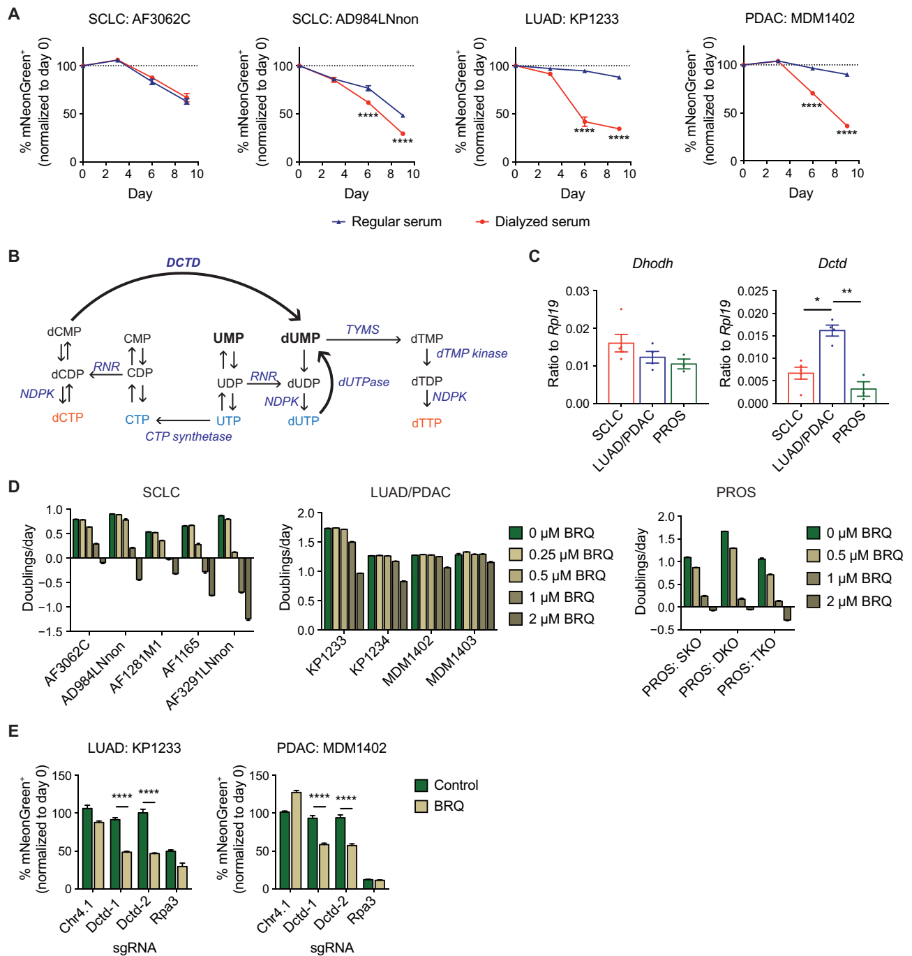
Fig. 3. LUAD/PDAC cells use alternative pathways to replenish cellular pyrimidine pools. (A) In vitro competition assays for SCLC, LUAD, and PDAC cell lines transduced with sgDhodh, grown in cell culture medium supplemented with either regular (nondialyzed) serum or dialyzed serum. Data are normalized to the transduction efficiency at day 0 ( n = 3 technical replicates for each sample). Data are presented as means \pm SEM. **** P < 0.0001 , two-way ANOVA with Sidak's multiple comparison test. (B) Pyrimidine nucleotide synthesis pathway. RNR, ribonucleotide reductase; TYMS, thymidylate synthetase; NDPK, nucleoside diphosphate kinase. (C) RNA expression of Dhodh (left) and Dctd (right) in SCLC, LUAD/PDAC, and prostate cancer (PROS) cell lines, as assessed by quantitative polymerase chain reaction (qPCR). Each point represents the mean of three technical replicates for one cell line. n = 5 cell lines for SCLC, n = 4 cell lines for LUAD/PDAC (2 each), and n = 3 cell lines for PROS. Data are presented as means \pm SEM. * P < 0.05 and ** P < 0.01 , Mann-Whitney test. (D) Quantification of PD rates for SCLC, LUAD/PDAC, and PROS cell lines treated with the indicated concentrations of brequinar ( n = 3 technical replicates per condition). For PROS cell lines, SKO: Pten -/- SKO prostate adenocarcinoma; DKO: Pten -/- ; Rb1 -/- DKO prostate neuroendocrine tumor; TKO: Pten -/- ; Rb1 -/- ; Trp53 -/- TKO prostate neuroendocrine tumor. Data are presented as means \pm SEM. (E) In vitro competition assays for LUAD (left) and PDAC (right) cell lines transduced with the indicated sgRNAs in the absence (green bars) and presence (brown bars) of brequinar (1 \mu M for KP1233; 2 \mu M for MDM1402). Data are normalized to the transduction efficiency at day 0 ( n = 3 technical replicates for each sample). Control cells were analyzed at day 3, and brequinar-treated cells were analyzed at day 4. Different days were chosen because of the decrease in rate of cell proliferation resulting from brequinar treatment (see main text and fig. S5). Data are presented as means \pm SEM. **** P < 0.0001 , two-way ANOVA with Sidak's multiple comparison test.
