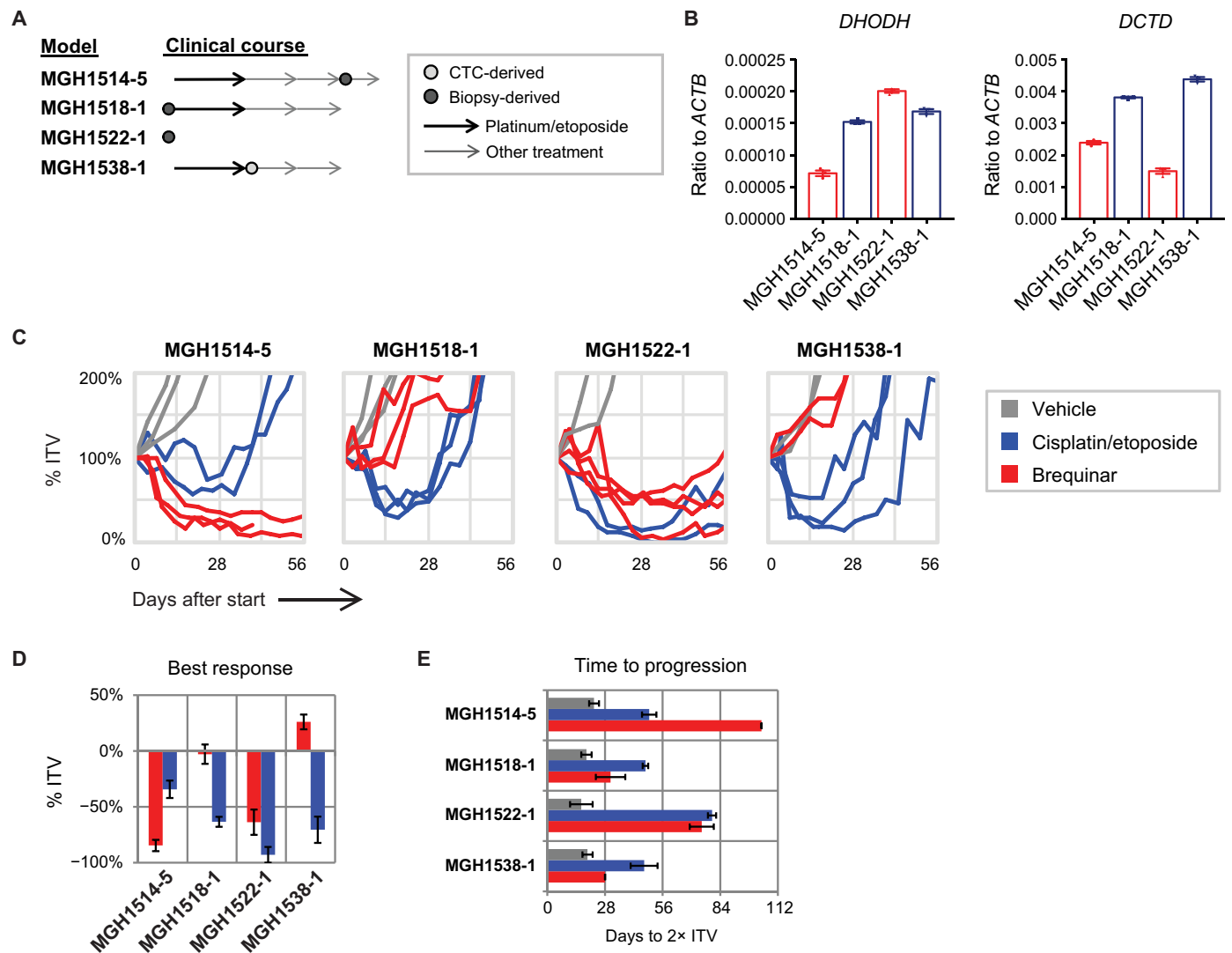
Fig. 5. PDX models of SCLC are sensitive to brequinar treatment. (A) Clinical time point and source of derivation for four SCLC PDX models treated with brequinar. Two models were derived from chemo-naïve patients, and two were derived after one or more lines of therapy. CTC, circulating tumor cell. (B) RNA expression of DHODH (left) and DCTD (right) in the four PDX models, as assessed by qPCR ( n = 3 technical replicates per sample). Data are presented as means \pm SEM. (C) Spider plots of xenograft volume versus time after start of treatment with brequinar, cisplatin/etoposide, or vehicle. Each line represents a single animal. % ITV, % initial tumor volume. Cisplatin/etoposide treatment data were obtained from Drapkin et al. (37). (D) Maximum xenograft regression for each model after day +7. Data are presented as means \pm SEM. (E) Time (days) from start of treatment to progression, which is defined as the point at which tumors reach twice of the initial tumor volume (2x ITV). Data are presented as means \pm SEM.
